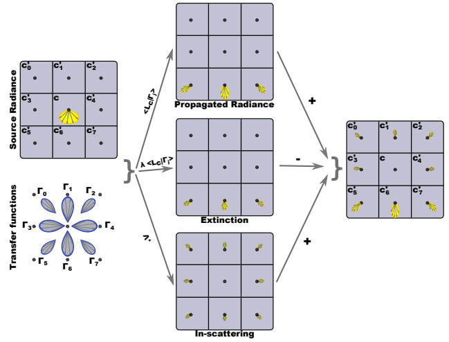
Figure 3: Illustration of propagation scheme described by Equation (3). Initially, only cell c contains radiance (top left). Using the transfer functions \Gamma_j (bottom left), radiance is then propagated from c to its neighbors c'_j . The propagation consists of three components: transferred radiance (top middle), extinction (center) and in-scattering (bottom middle). Summing these contributions yield the radiance distribution (right side). This radiance distribution is scaled using the blocking factors b_{cc'} (not shown in figure). Without scattering, the cells c'_0 through c'_4 would never receive any radiance.
